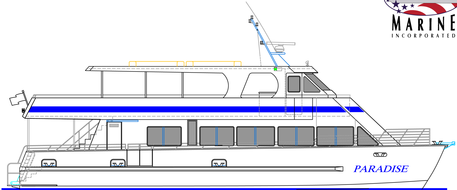
Outboard Profile
