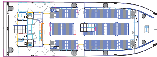
MAIN DECK ARRANGEMENT
