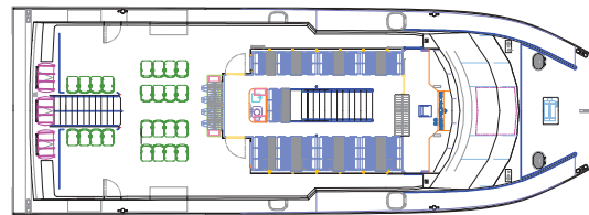
UPPER DECK ARRANGEMENT
