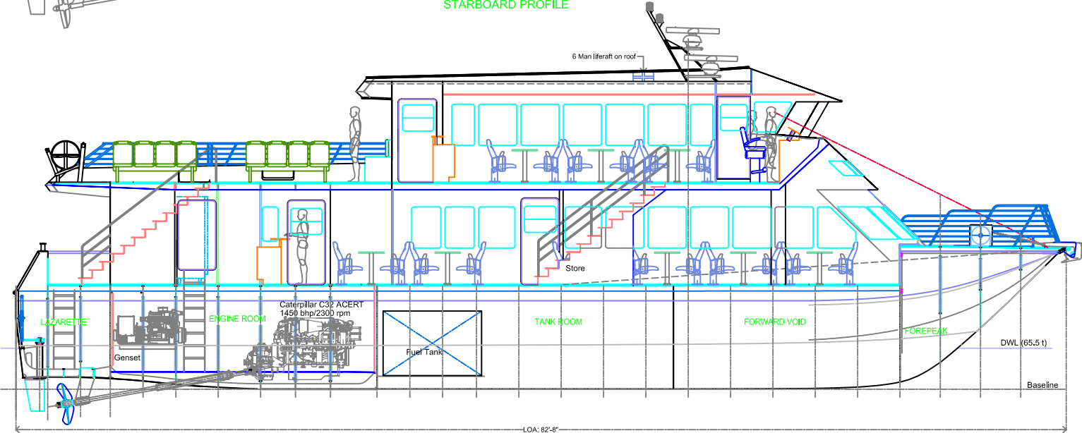
LONGSECTION (SCHEMATIC)
