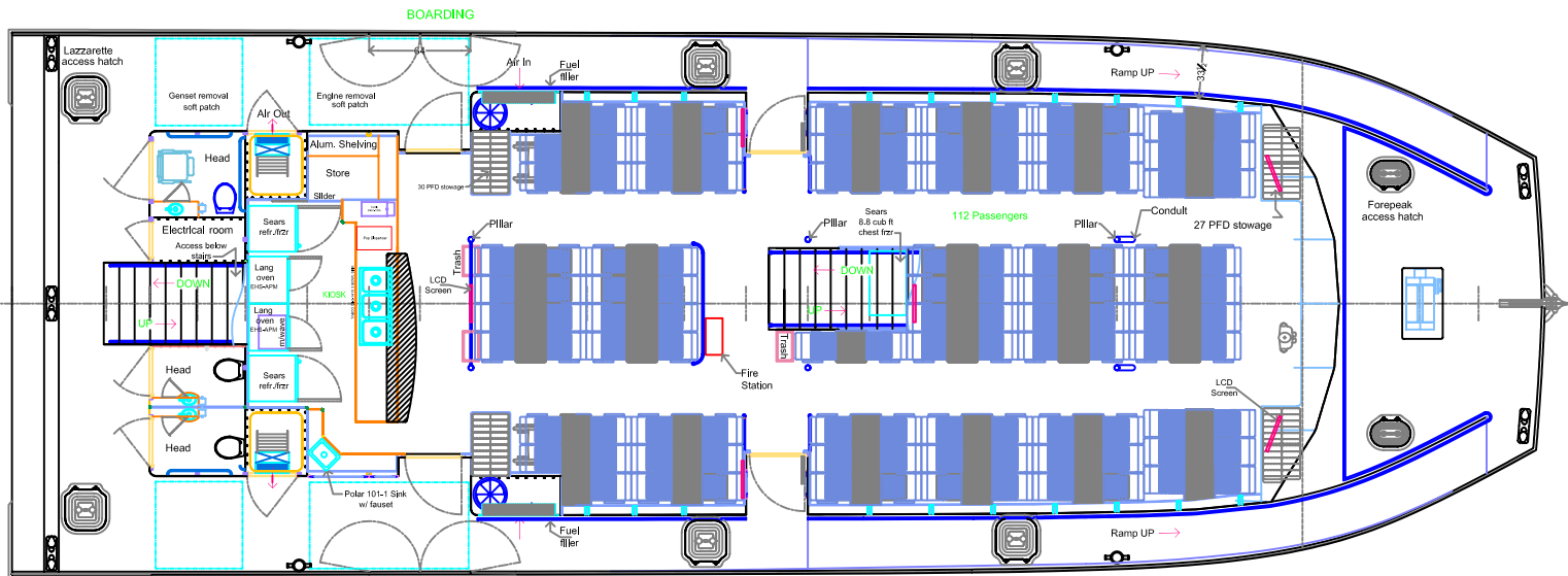
MAIN DECK ARRANGEMENT
