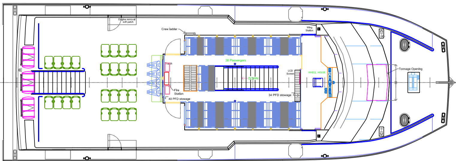
UPPER DECK ARRANGEMENT
