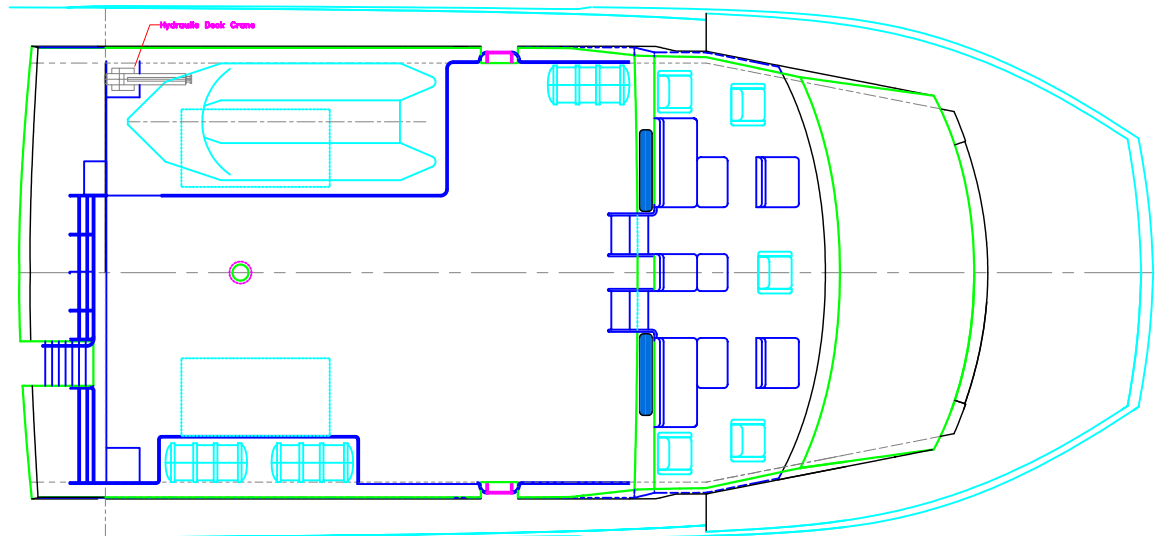
UPPER DECK ARRANGEMENT
