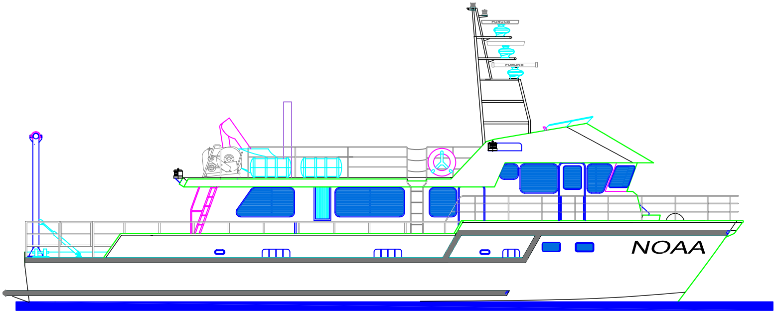
OUTBOARD PROFILE
