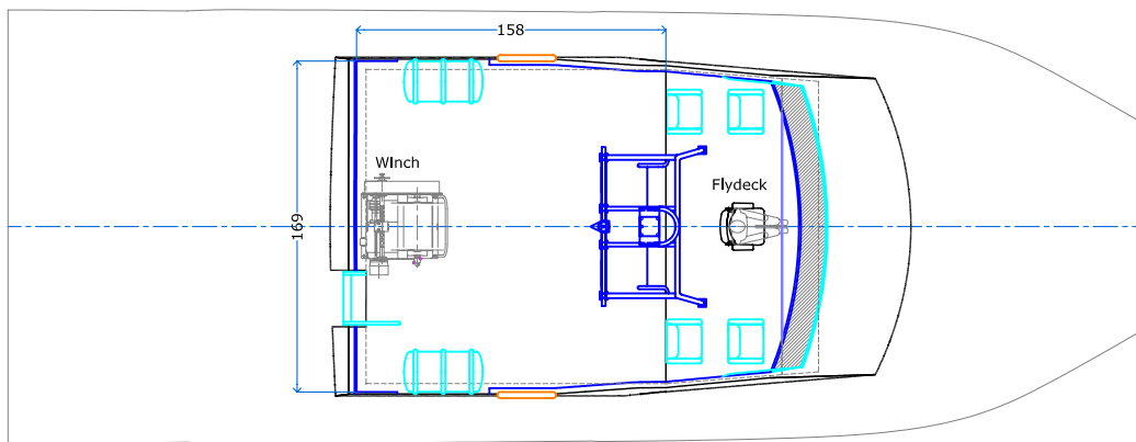
UPPER DECK ARRANGEMENT
