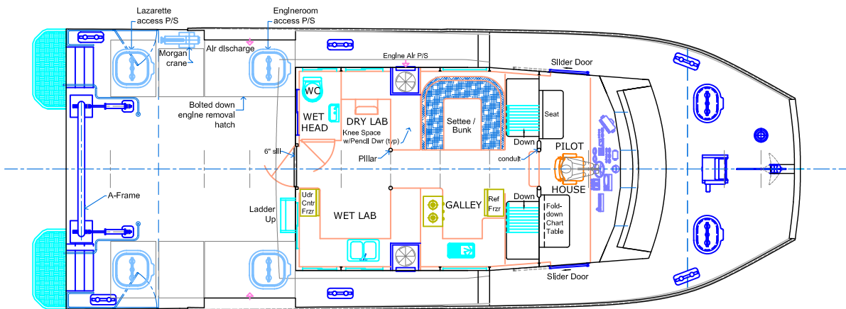
MAIN DECK ARRANGEMENT
