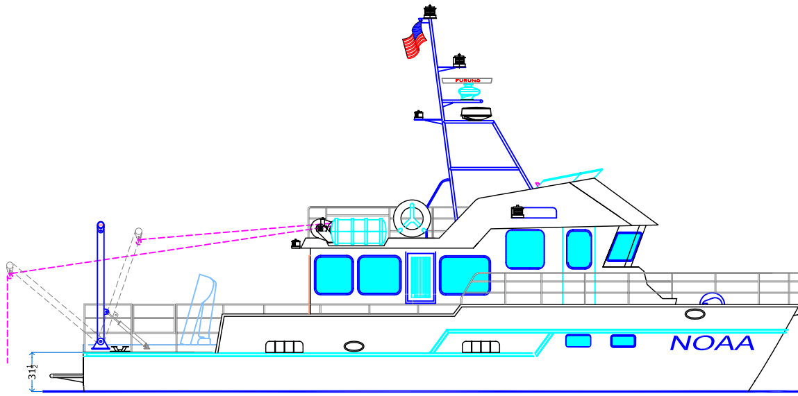
OUTBOARD PROFILE
