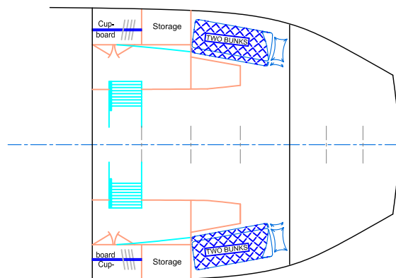
ACCOMMODATION DECK ARRANGEMENT
